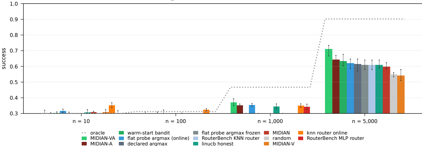
RouterEval real LLM pools, all_weak (10-1,000) + leaderboard (5,000), \beta = 0.5 , low-skill cartel
