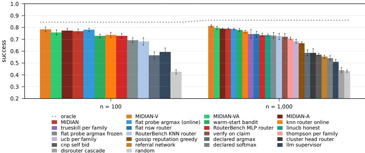
live RTE, specialist, \beta = 0.1 , random liars
