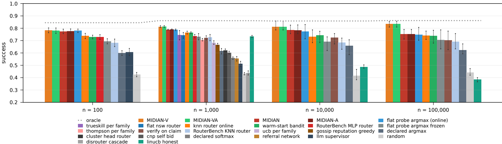
live RTE, specialist, honest ( \beta = 0 )
