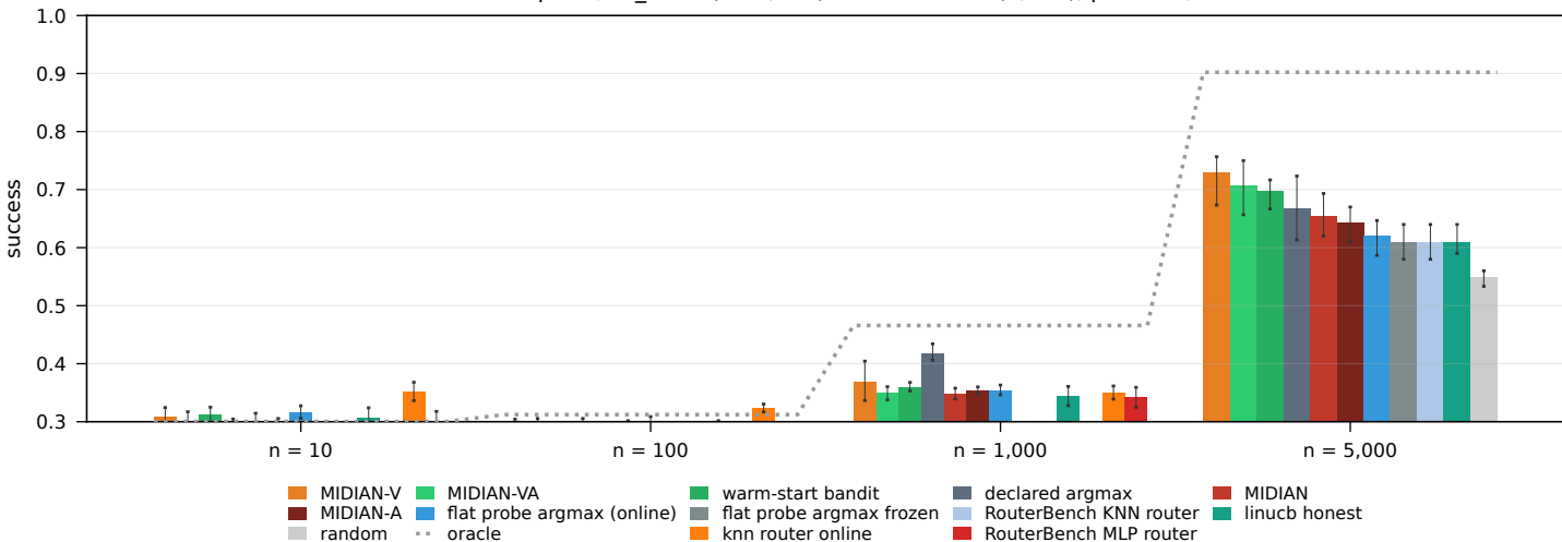
RouterEval real LLM pools, all_weak (10-1,000) + leaderboard (5,000), \beta = 0.25 , random liars
