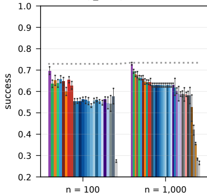
live RTE, heavy_tail, \beta = 0.25 , random liars
