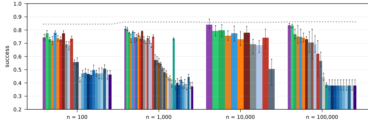
live RTE, specialist, \beta = 0.5 , random liars
