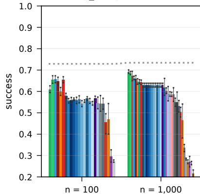
live RTE, heavy_tail, \beta = 0.5 , low-skill cartel
