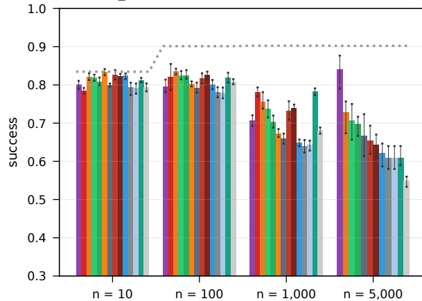
RouterEval real LLM pools, all_strong (10-1,000) + leaderboard (5,000), \beta = 0.25 , random liars
