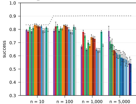
RouterEval real LLM pools, all_strong (10-1,000) + leaderboard (5,000), \beta = 0.5 , random liars
