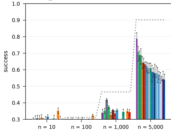
RouterEval real LLM pools, all_weak (10-1,000) + leaderboard (5,000), \beta = 0.5 , random liars
