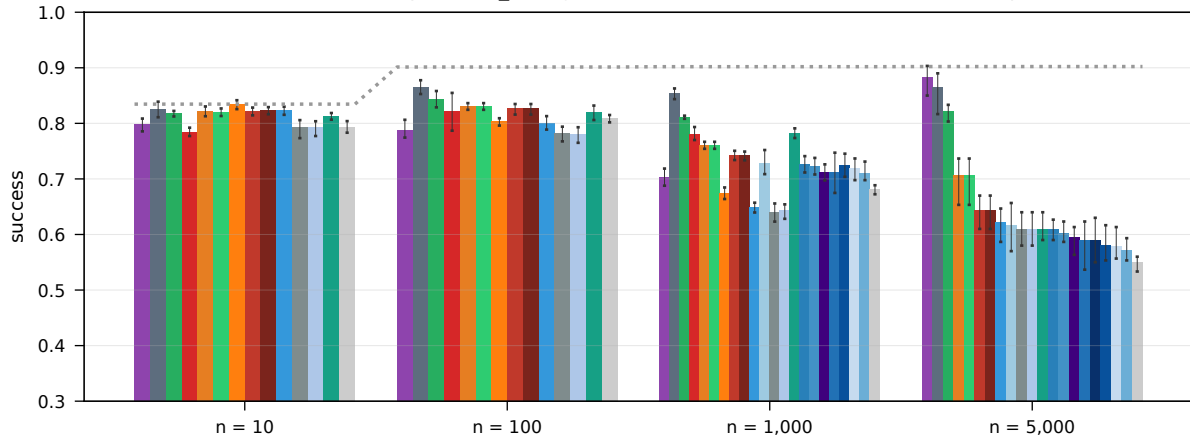
RouterEval real LLM pools, all_strong (10-1,000) + leaderboard (5,000), honest ( \beta = 0 )
