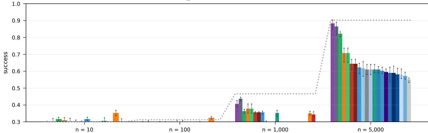
RouterEval real LLM pools, all_weak (10-1,000) + leaderboard (5,000), honest ( \beta = 0 )
