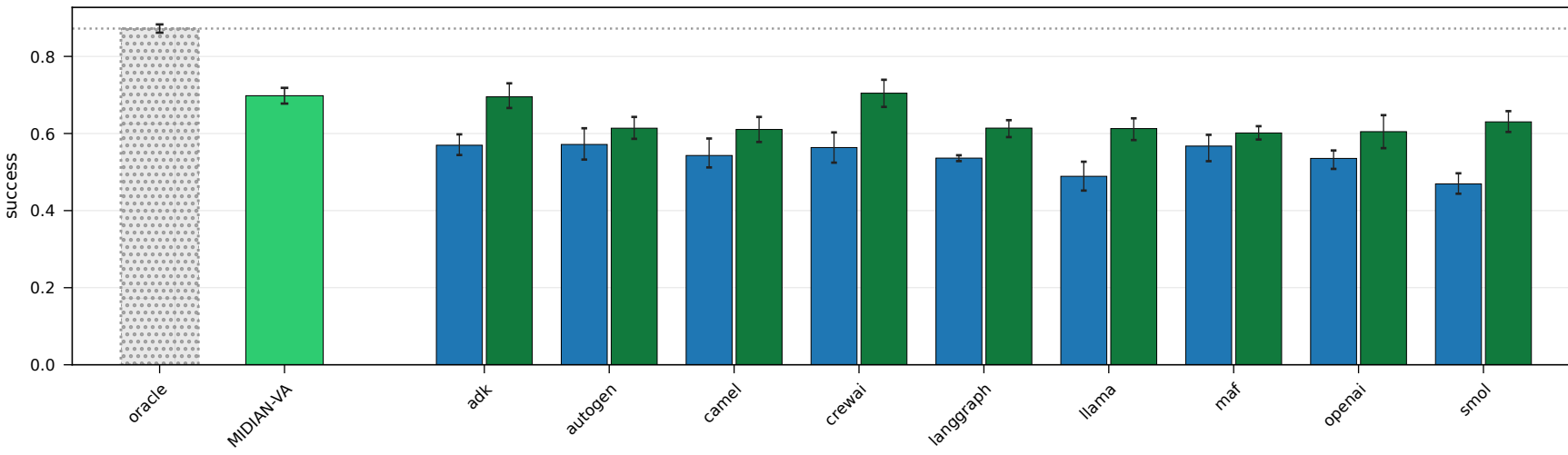
oracle MIDIAN-VA (whole population) MiniLM cosine MIDIAN-VA leaf cohort routrereval · n = 1,000 · strong_to_weak · \beta = 0.5 , random liars (9 frameworks × 2 shortlists, 5 seeds)
