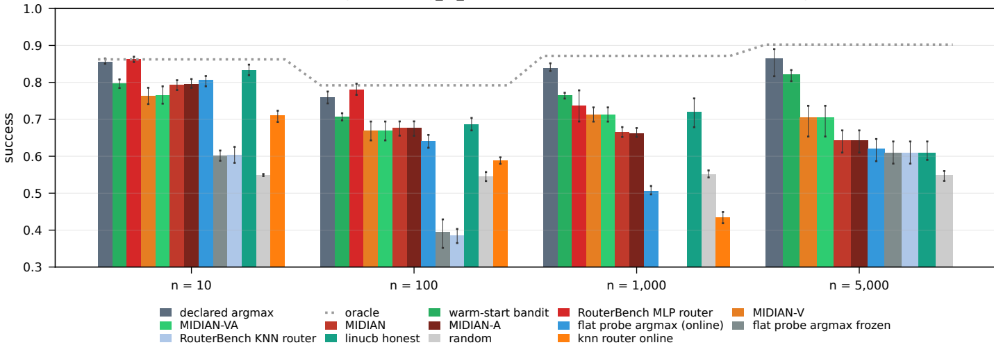
RouterEval real LLM pools, strong_to_weak (10-1,000) + leaderboard (5,000), honest ( \beta = 0 )
