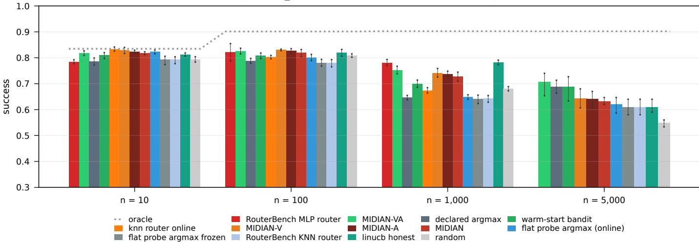
RouterEval real LLM pools, all_strong (10-1,000) + leaderboard (5,000), \beta = 0.5 , random liars
