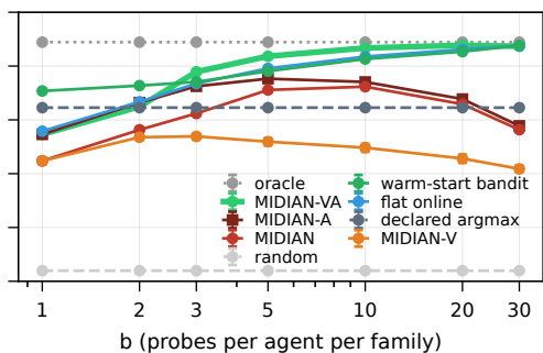
colluding low-skill cartel, \beta = 0.5
