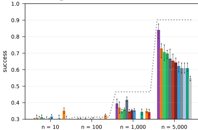
RouterEval real LLM pools, all_weak (10-1,000) + leaderboard (5,000), \beta = 0.25 , random liars
