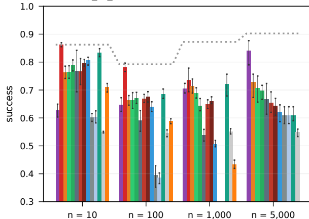
RouterEval real LLM pools, strong_to_weak (10-1,000) + leaderboard (5,000), \beta = 0.25 , random liars
