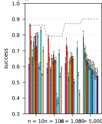
RouterEval real LLM pools, strong_to_weak (10-1,000) + leaderboard (5,000), \beta = 0.5 , random liars
