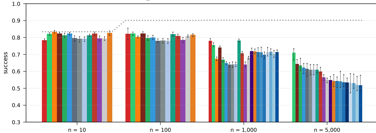
RouterEval real LLM pools, all_strong (10-1,000) + leaderboard (5,000), \beta = 0.5 , low-skill cartel
