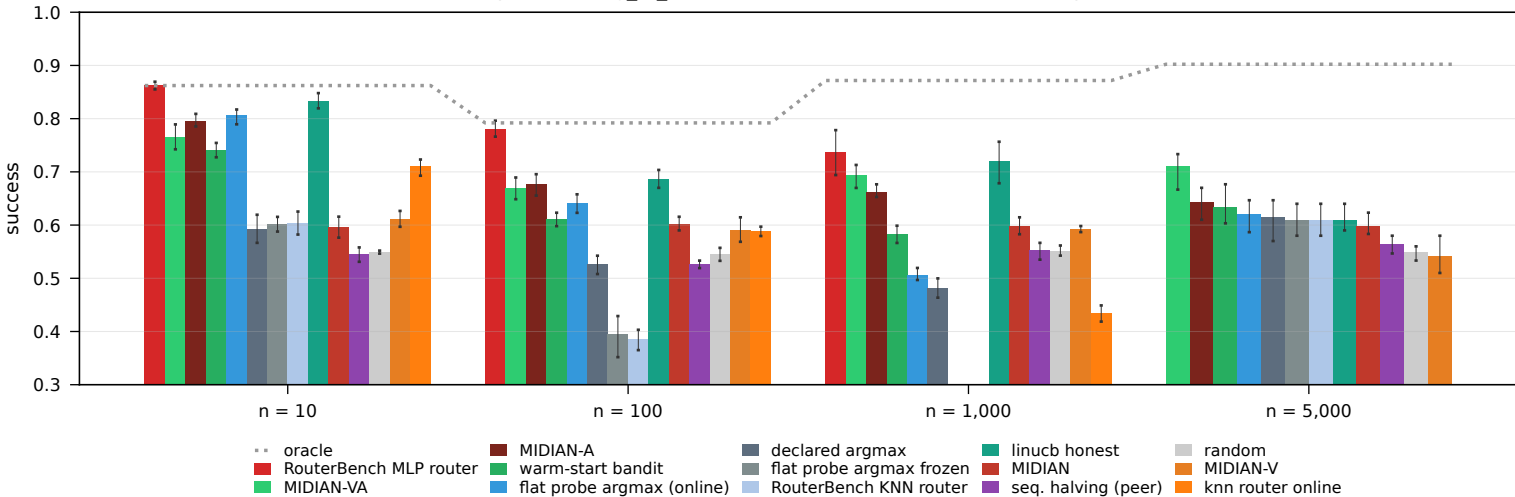
RouterEval real LLM pools, strong_to_weak (10-1,000) + leaderboard (5,000), \beta = 0.5 , low-skill cartel
