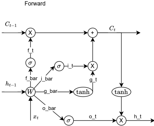
LSTM Cell
