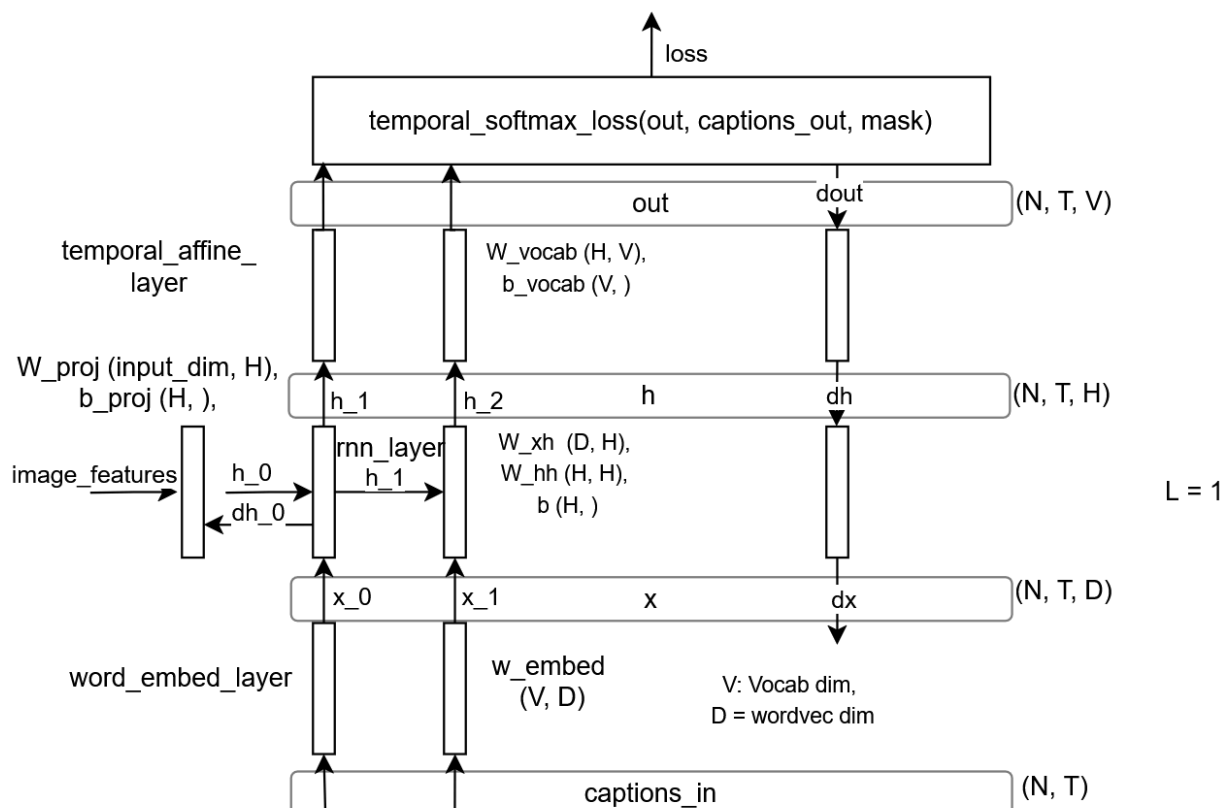
simple RNN Classifier for Image Captioning
