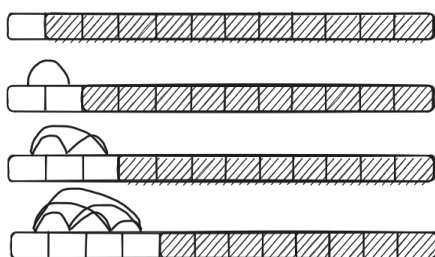
function of mask in decoder self-attention
