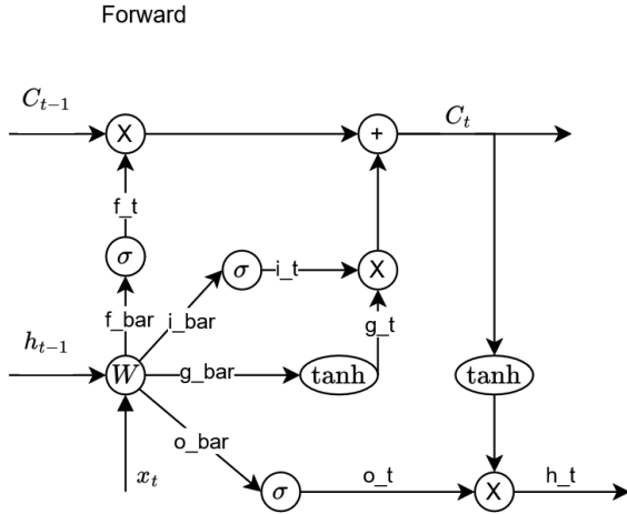
LSTM Cell
