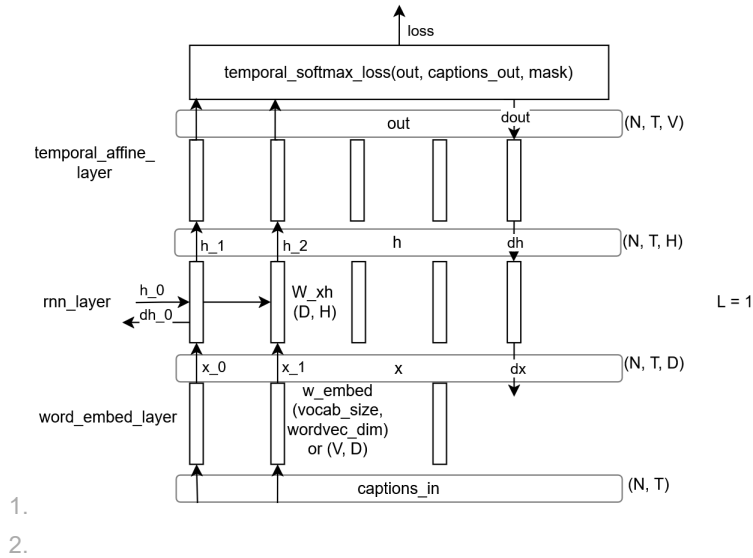
simple RNN Classifier for Image Captioning
