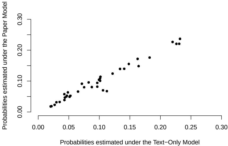
Figure 6: Comparing the predictions of the Paper Model and the Text-Only Model
