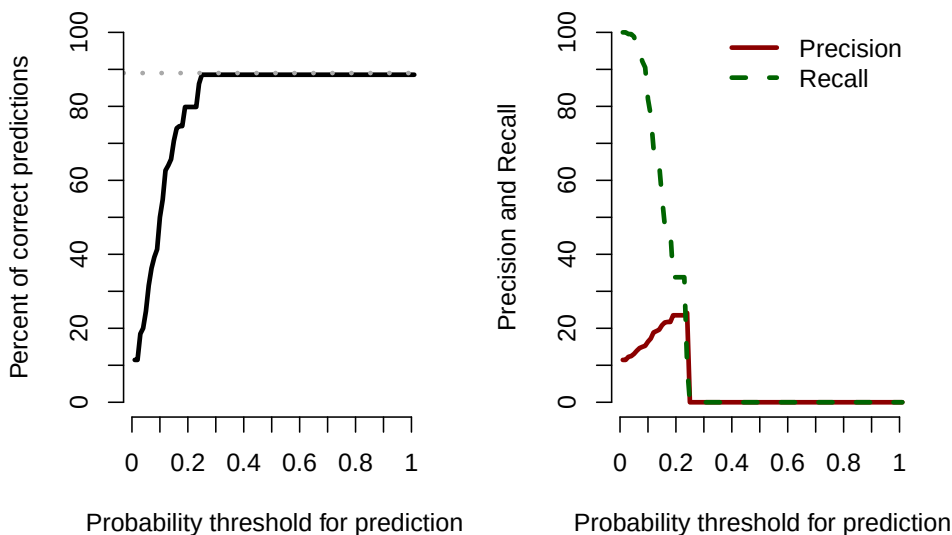
Figure 5: Left: Percent of binary predictions based on the Paper Model at varying thresholds; only for data used to estimate the model parameters and grouped by their actual outcome; Right: Precision and Recall for the Paper Model at varying thresholds; only for data used to estimate the model parameters and grouped by their actual outcome
