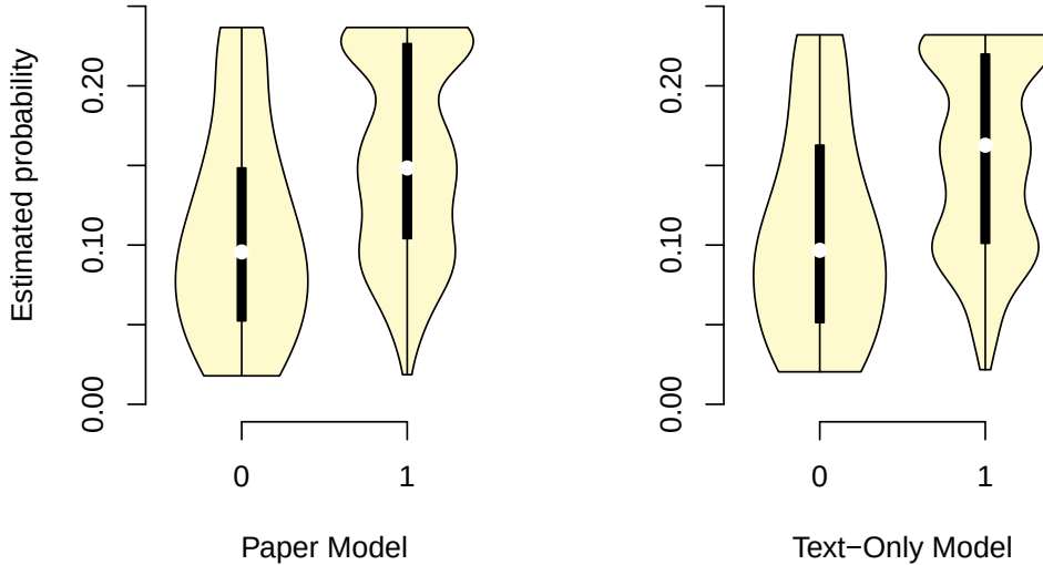
Figure 4: Probabilities estimated by the Paper Model and the Text-Only Model; only for data used to estimate the model parameters and grouped by their actual outcome
