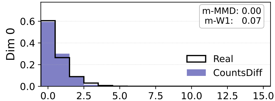
CountsDiff Joint-MMD: 0.001 Joint-SWD: 0.76
