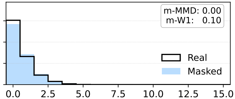
Masked Joint-MMD: 0.001 Joint-SWD: 1.47
