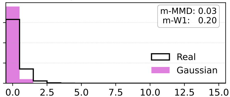
Gaussian Joint-MMD: 0.054 Joint-SWD: 1.17
