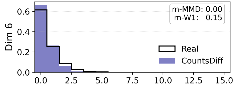
CountsDiff Joint-MMD: 0.001 Joint-SWD: 0.80
