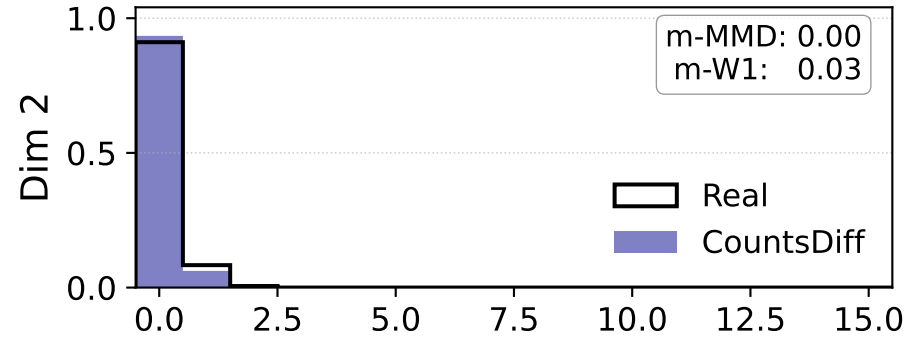
CountsDiff Joint-MMD: 0.001 Joint-SWD: 0.83
