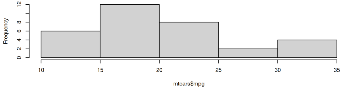
Histogram of mtcars$mpg
