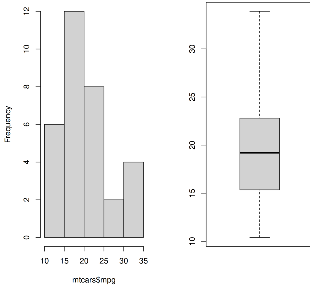
Histogram of mtcars$mpg
