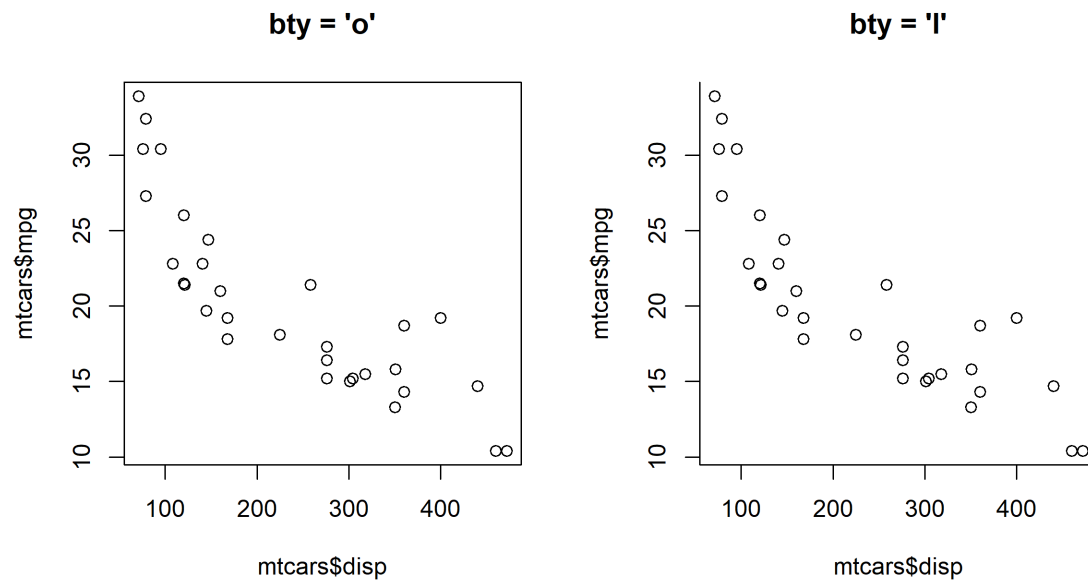
Figure 41: Effect of par(bty) on the box drawn around the plot
