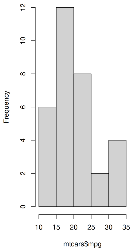
Histogram of mtcars$mpg
