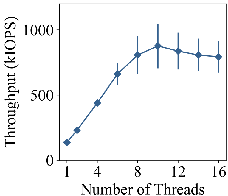
ext4 Random Write
