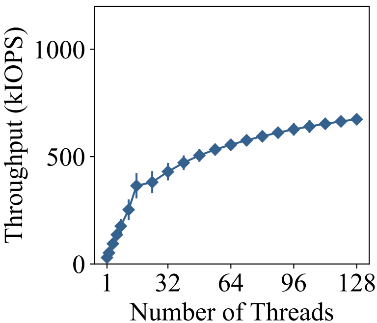
ext4 Random Read
