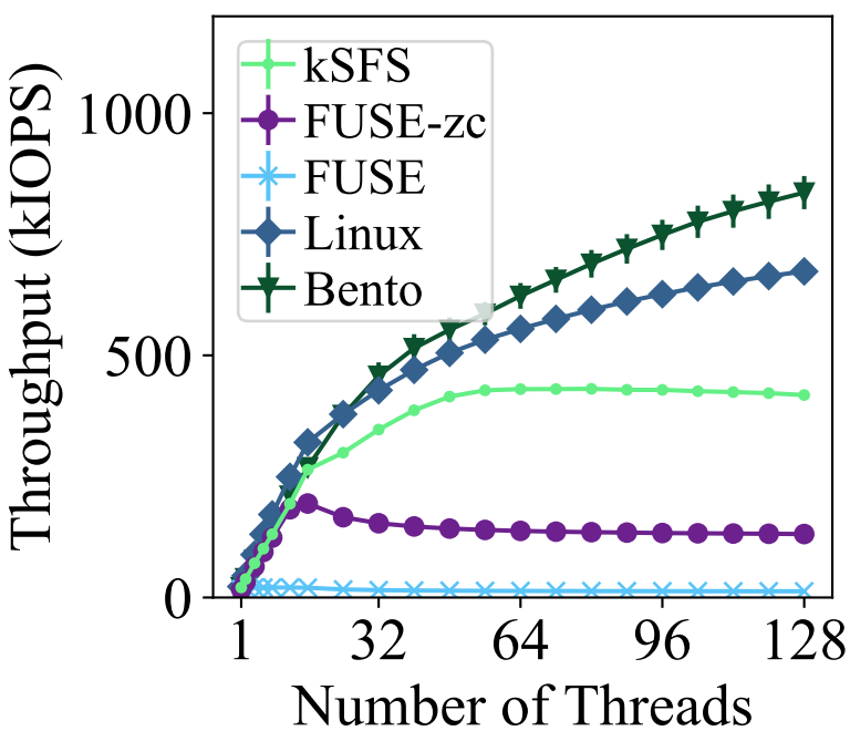
exFAT Random Read
