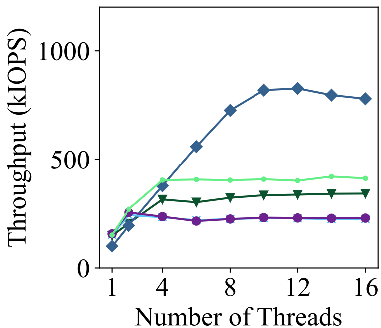
exFAT Random Write
