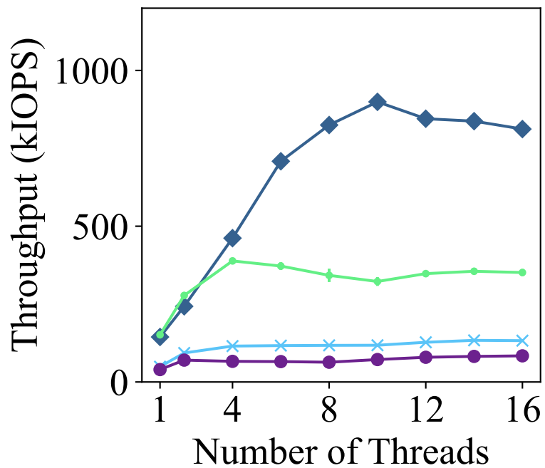
NTFS Random Write
