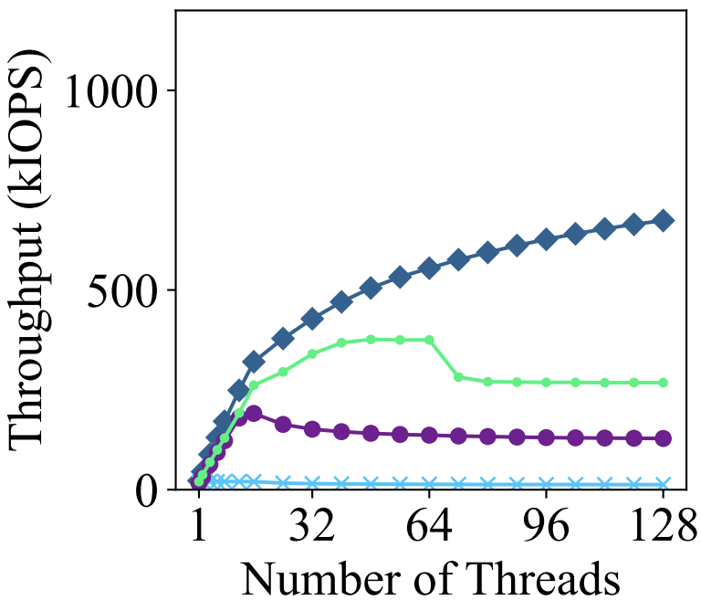
NTFS Random Read
