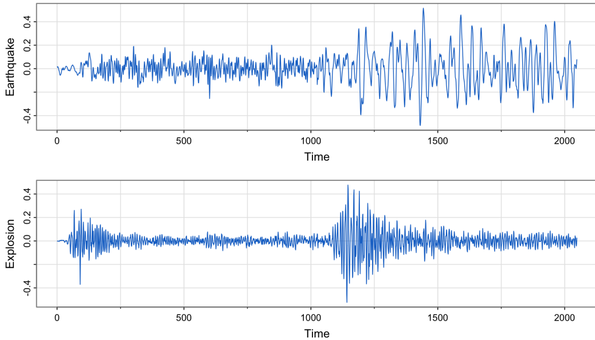
Figure 3: Arrival phases from an earthquake (top) and explosion (bottom) at 40 points per second.
