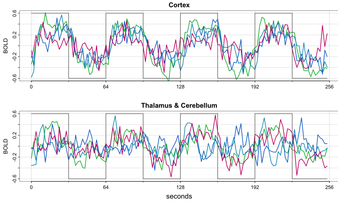
Figure 4: fMRI data from various locations in the cortex, thalamus, and cerebellum; n = 128 points, one observation taken every 2 seconds.
