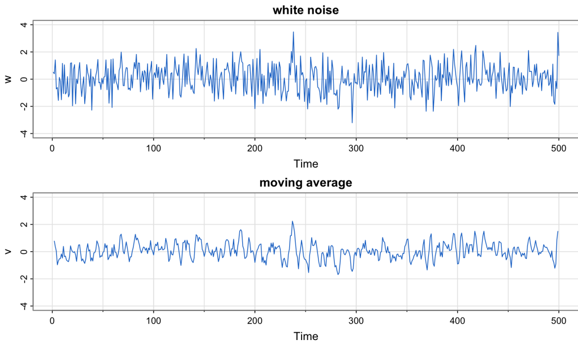
Figure 5: Gaussian white noise series (top) and three-point moving average of the Gaussian white noise series (bottom).
