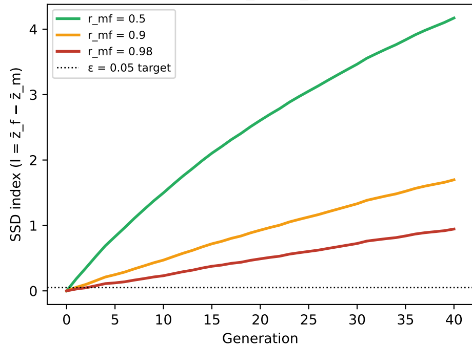
A. Effect of r_{mf} ( N_e = 10^4 )
