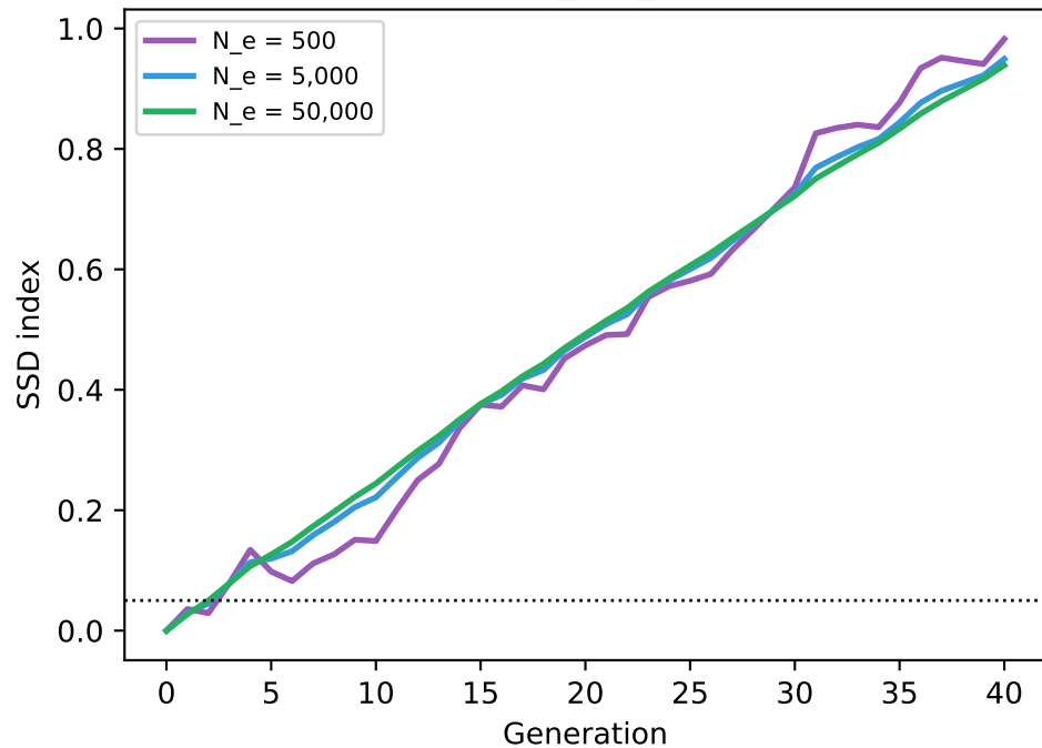
B. Effect of N_e ( r_{mf} = 0.98 )
