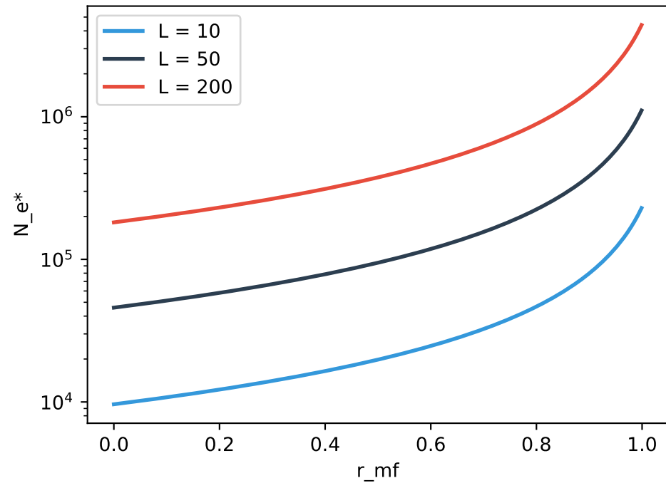
Sensitivity to locus number L
