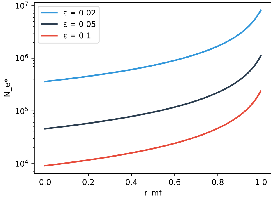
Sensitivity to accuracy target \varepsilon
