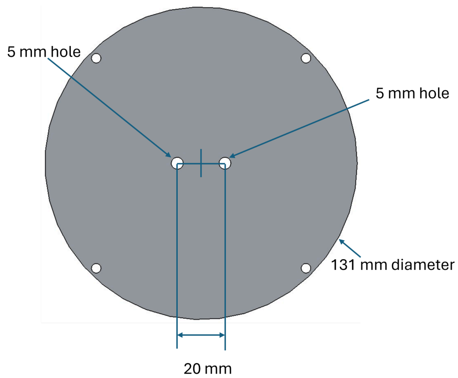
Container Bottom Disk Dimensions
