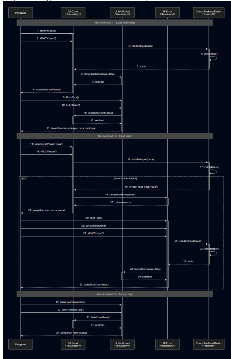
Gambar 3. 9 Seq Diagram#4: Alternative Flow
