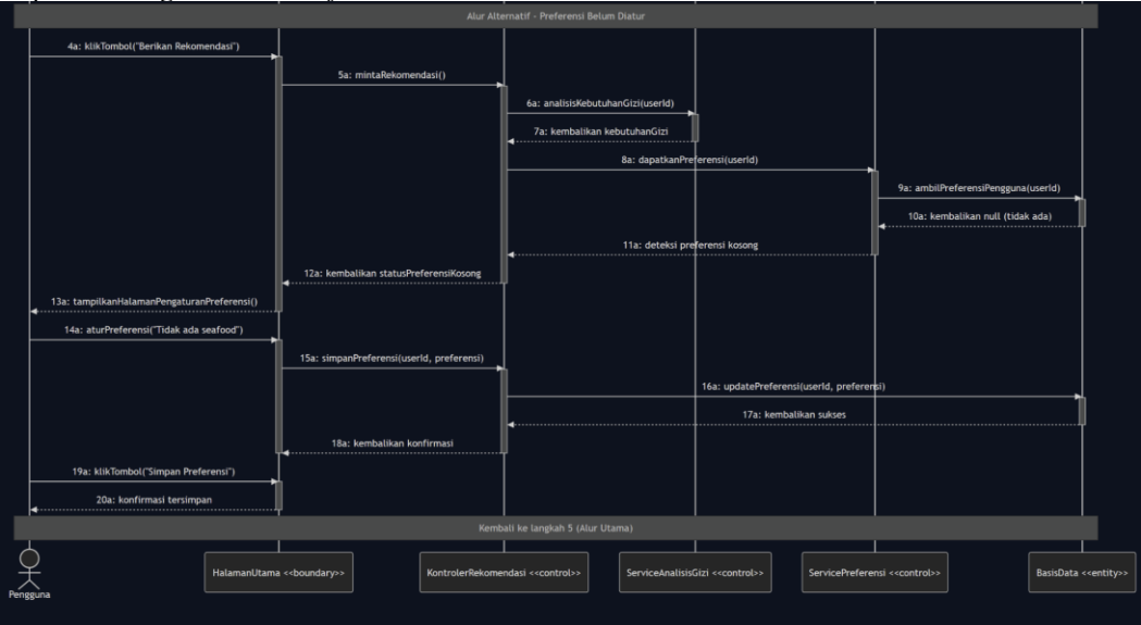
Gambar 3. 5 Seq Diagram#2: Alternative Flow
