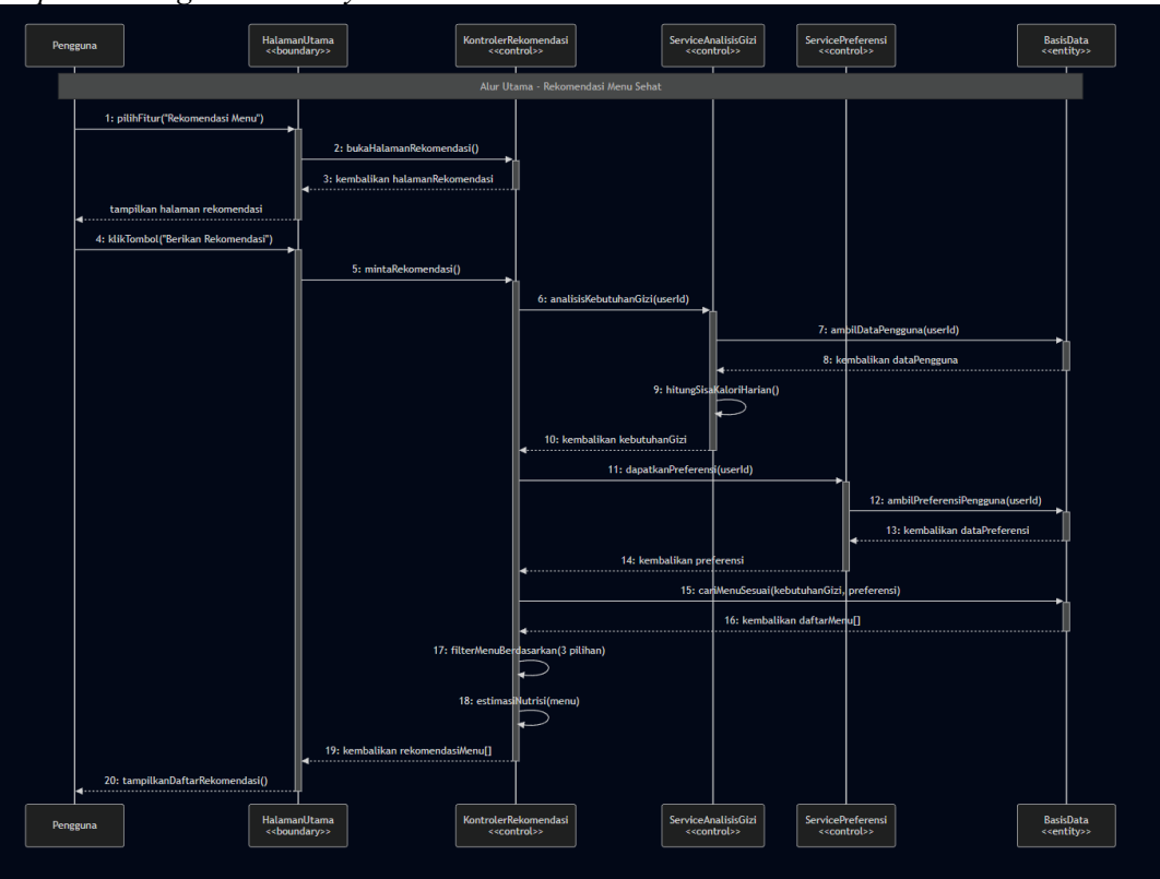
Gambar 3. 4 Seq Diagram#2: Primary Flow
