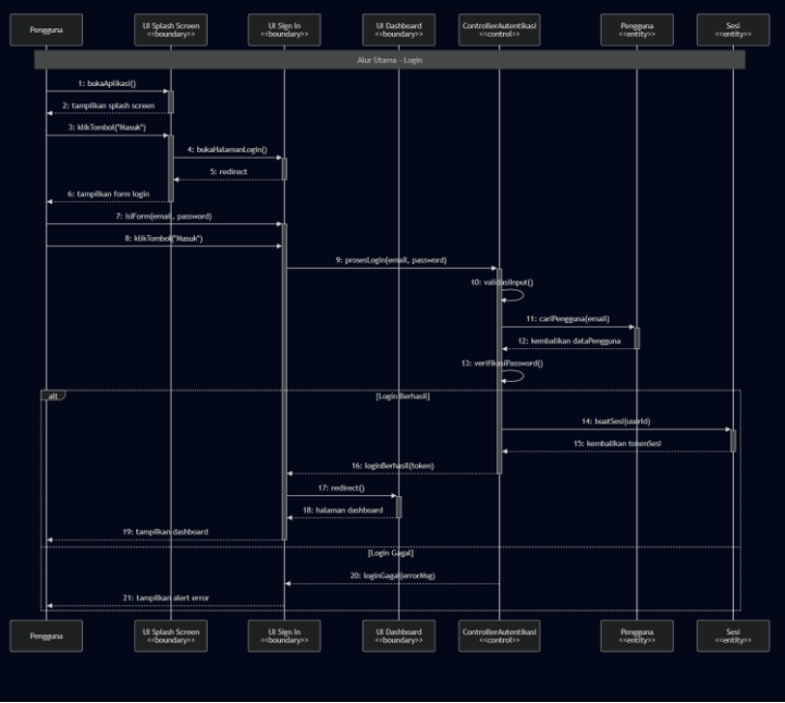
Gambar 3. 6 Seq Diagram#3: Sign In
