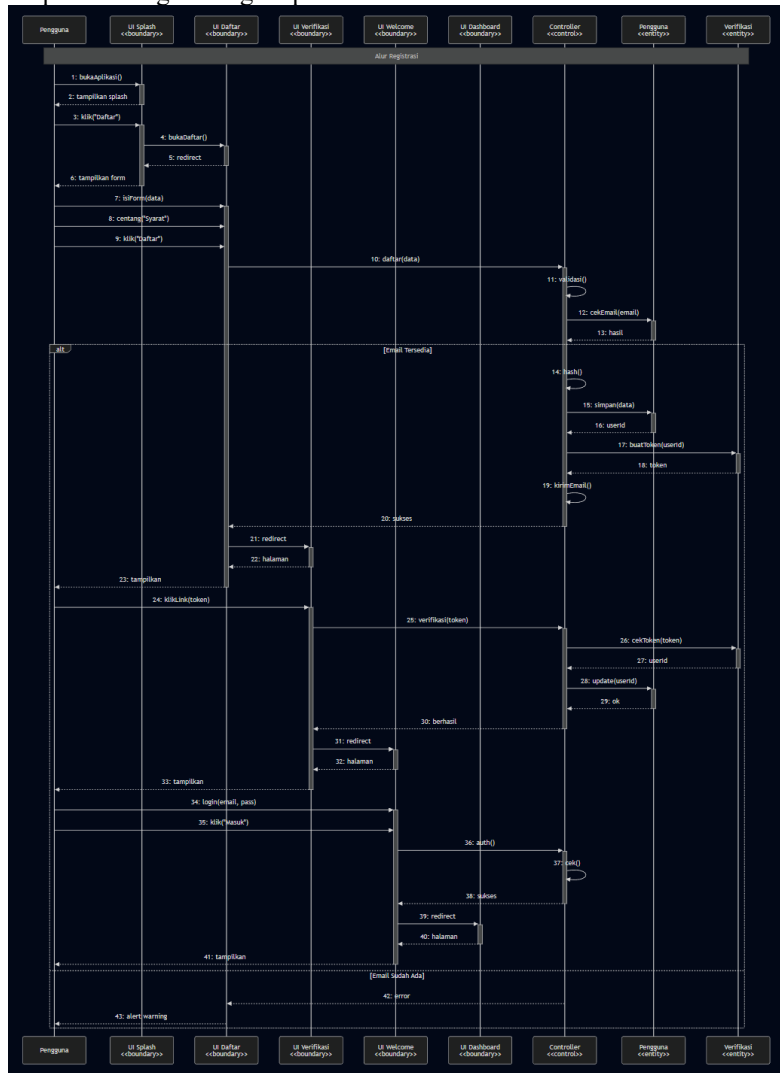
Gambar 3. 7 Seq Diagram#3: Sign Up
