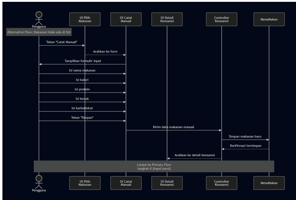
Gambar 3. 3 Seq Diagram#1: Alternative Flow
