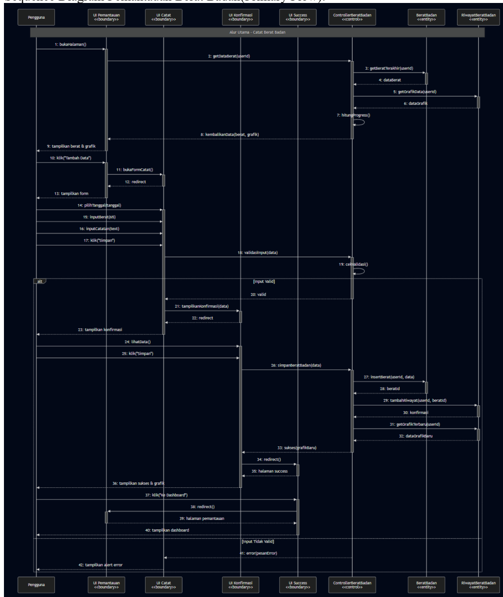
Gambar 3. 8 Seq Diagram#4: Primary Flow
