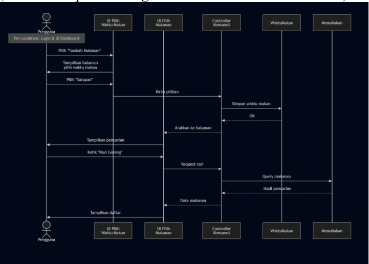
Gambar 3. 1 Sequence Diagram#1 (Part1)
