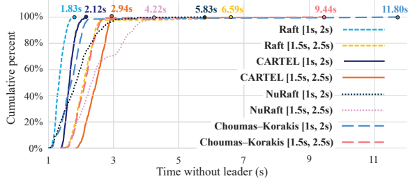
Fig. 6: Cumulative percentage plot of time without a leader
