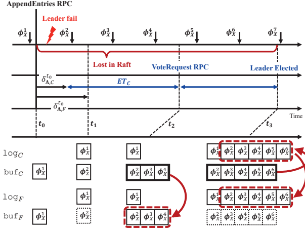
Fig. 4: Functionality of CARTEL node buffer
