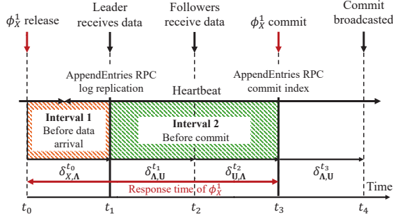
Fig. 1: Response time of data in Raft
