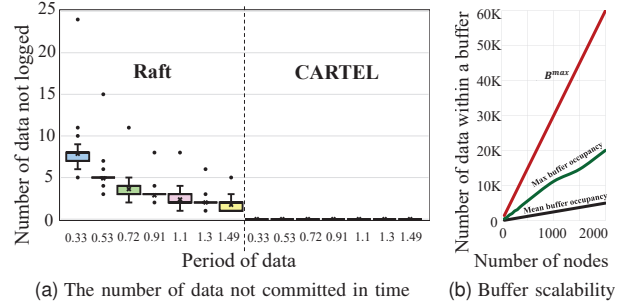
Fig. 7: Experiment and simulation results
