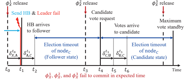
Fig. 2: Raft operation of leader election
