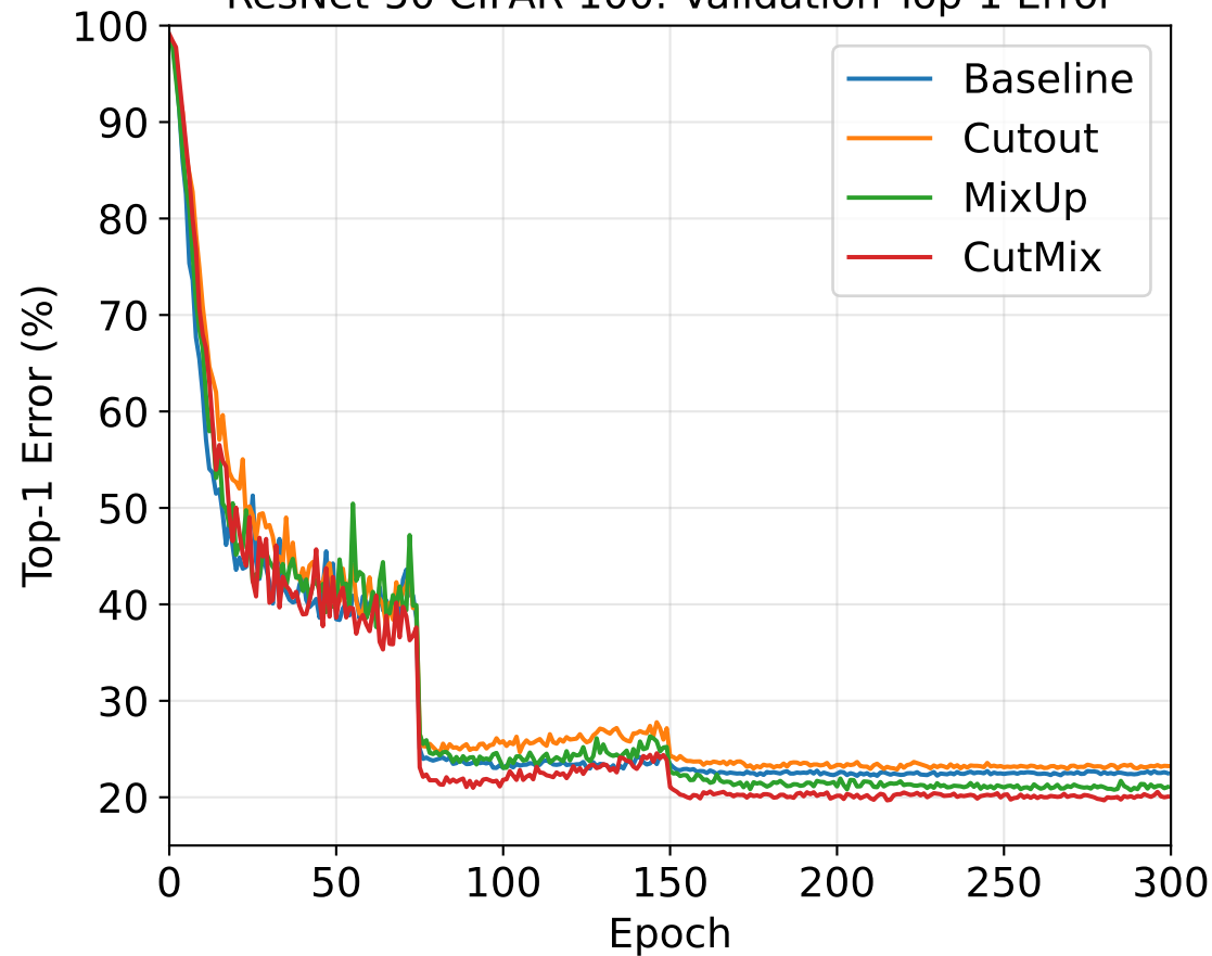
ResNet-50 CIFAR-100: Validation Top-1 Error
