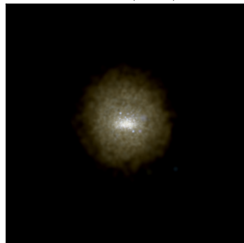
2cDM (-2,-2)
