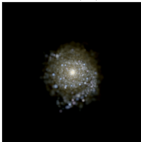
2cDM (0,0)
