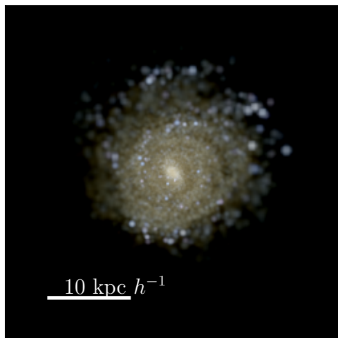
CDM
