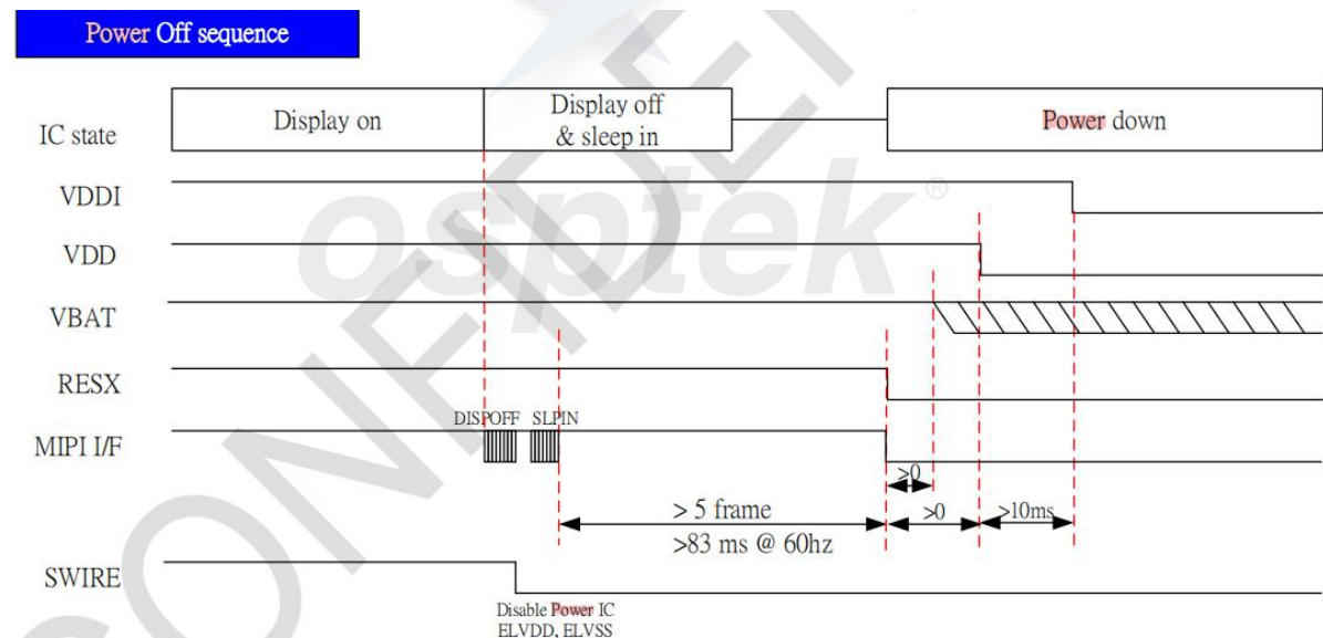
Figure 10 Power Off Sequence
