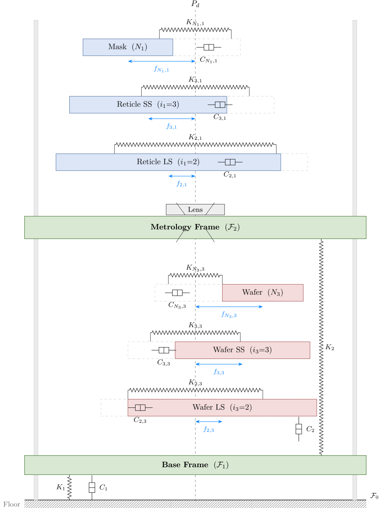
Figure 1: Lumped-parameter mechatronic model of the lithography step-and-scan tool, following [?]. The dashed vertical line is the intended trajectory P_d . Each stage block is offset from P_d by its generalised in-plane displacement f_{i,j} (blue double-headed arrows). Horizontal Kelvin–Voigt
