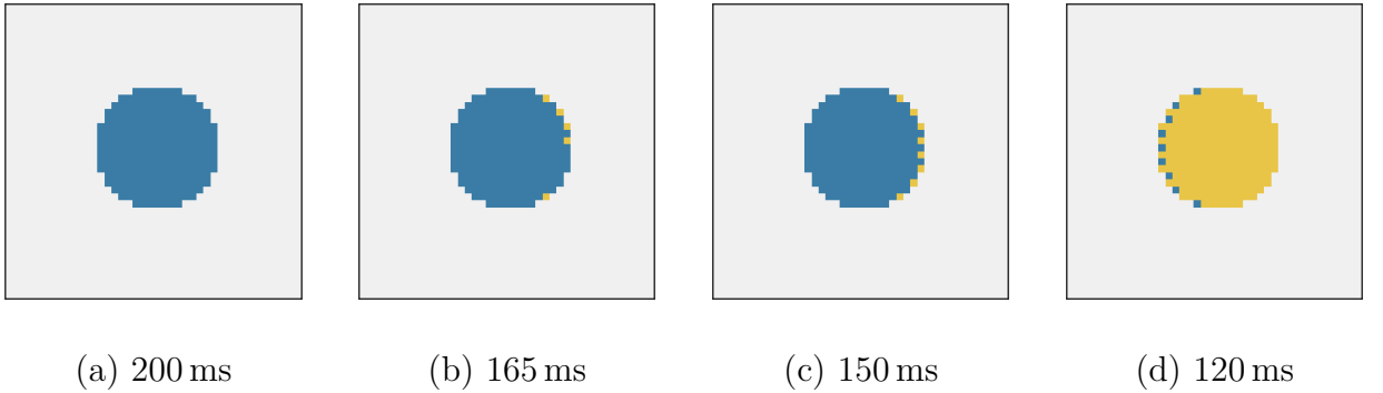
Figure 5.10: Wafer maps across the throughput–yield transition. At 165 ms the first failures form an edge cluster at the row-change dies; the cluster persists through 150 ms; by 120 ms failure is near-total and the map saturates.
