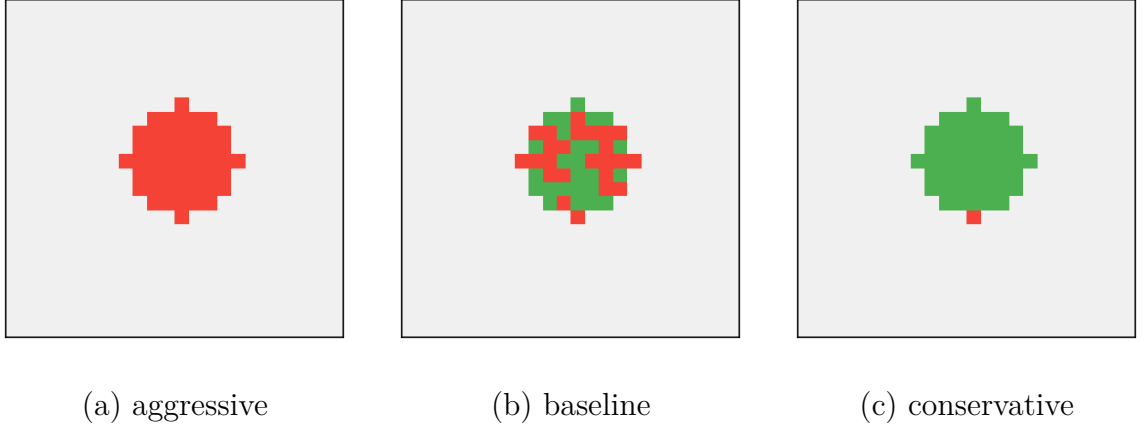
Figure 5.8: Simulated wafer maps under the representative setups (green: passing, red: failing).
