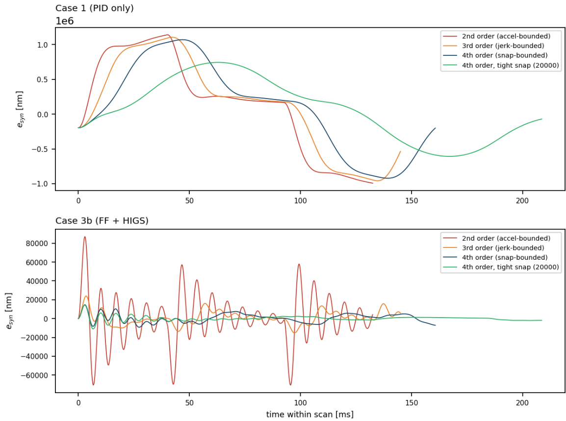
Figure 5.12: Synchronization error during one scan for the four profile orders, under bare Case 1 (top) and Case 3b (bottom).
