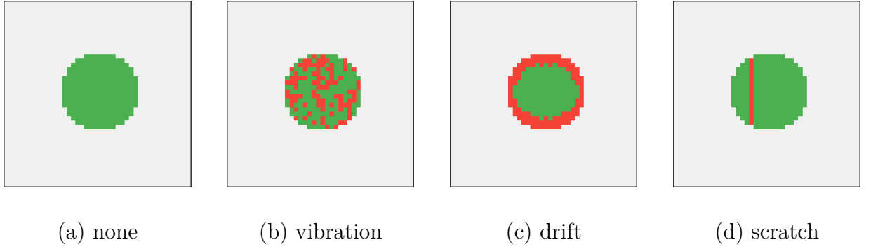
Figure 5.7: Simulated wafer maps under the four conditions (green: passing, red: failing).
