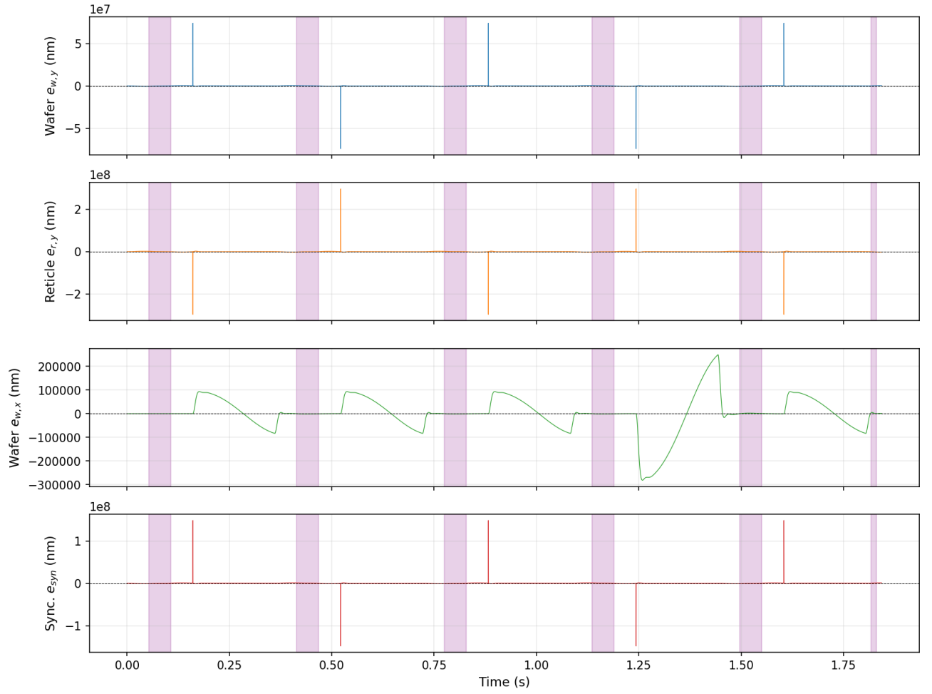
Figure 5.2: Wafer, reticle, and synchronization errors. Shaded bands mark the exposure windows.
