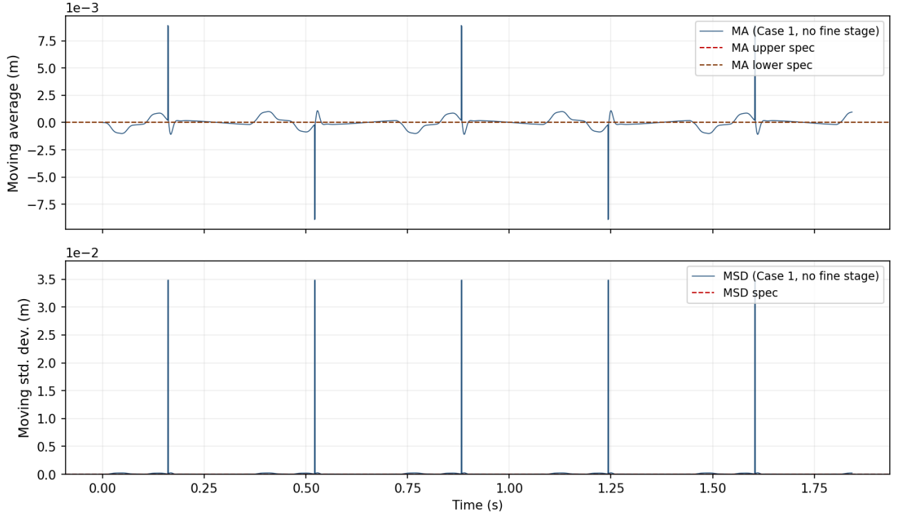
Figure 5.4: MA and MSD performance indices of the synchronization error.
