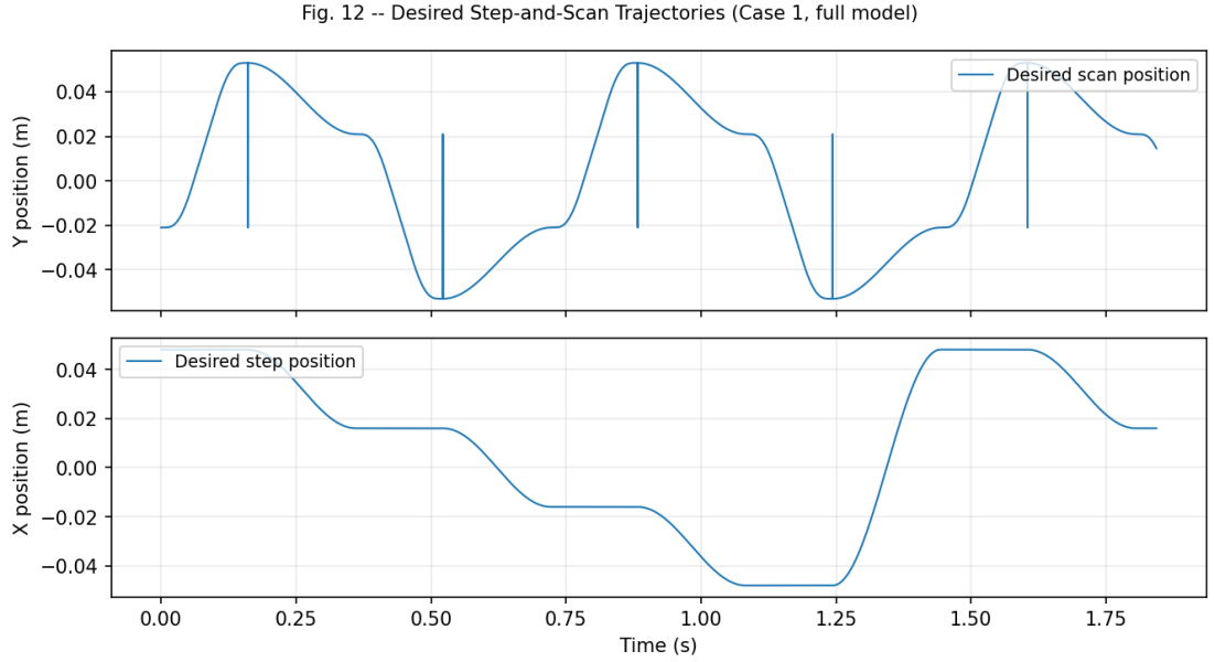
Figure 5.1: Commanded step-and-scan references for the wafer stage ( x : stepping, y : scanning) over the four-die sequence.
