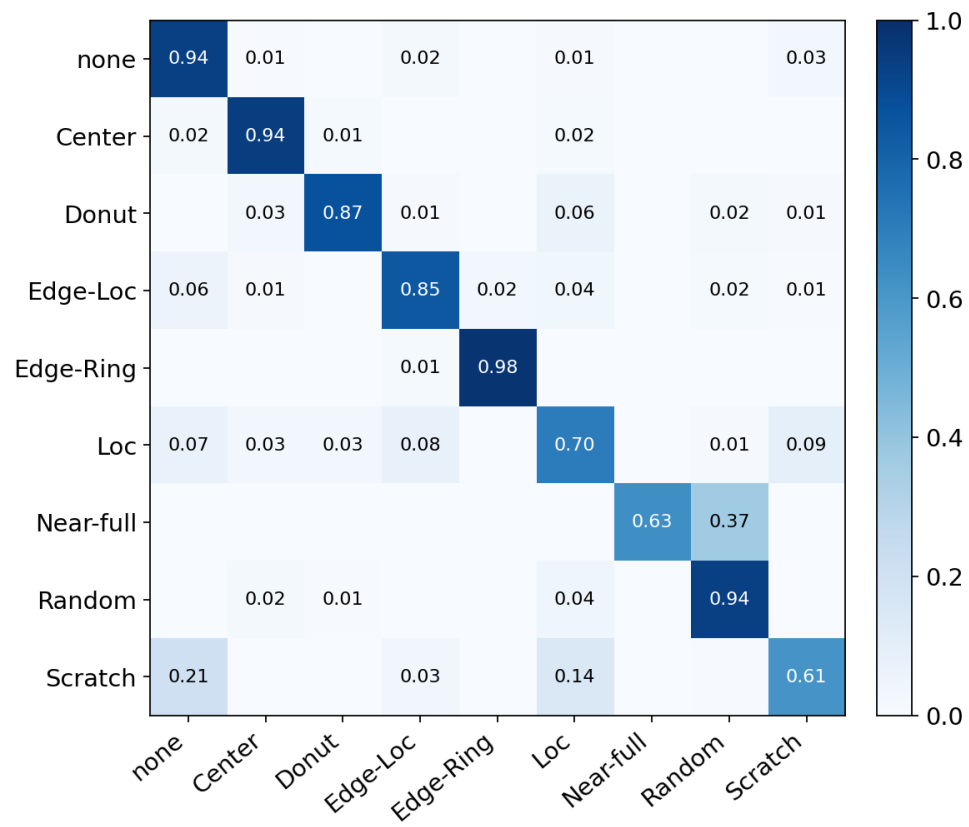
Figure 5.6: Row-normalized confusion matrix of the class-weighted model.
