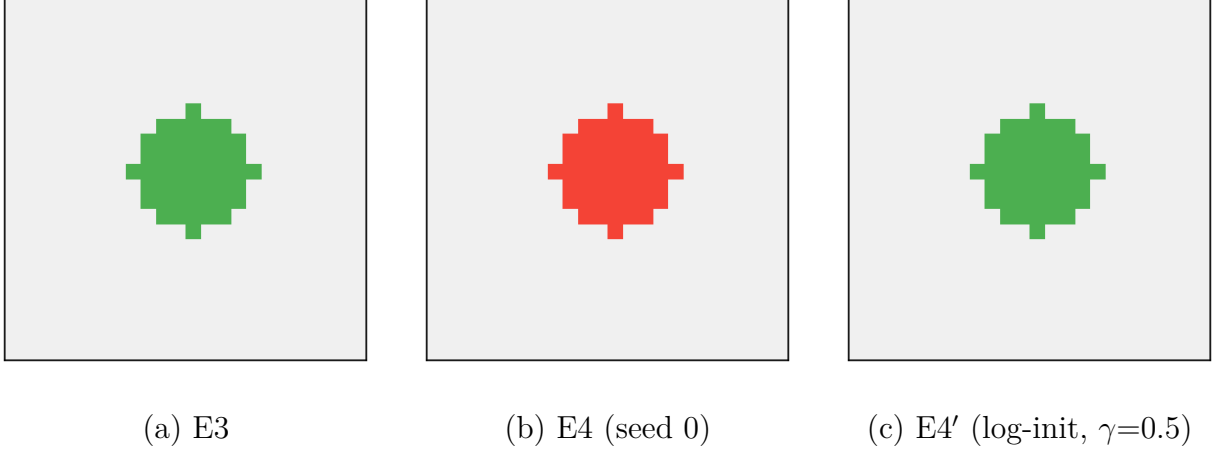
Figure 5.11: Best-particle wafer maps found by the optimization scenarios (green: passing, red: failing). The servo-cost search (E3) converges to a fully clean wafer; the CNN-cost search under the original linear-uniform initialization and \gamma = 1 (E4) remains fully saturated on the Center -classified plateau, identically for both tested random seeds; log-uniform initialization with \gamma = 0.5 (E4') converges to a fully clean wafer as well (Table 5.7.1).
