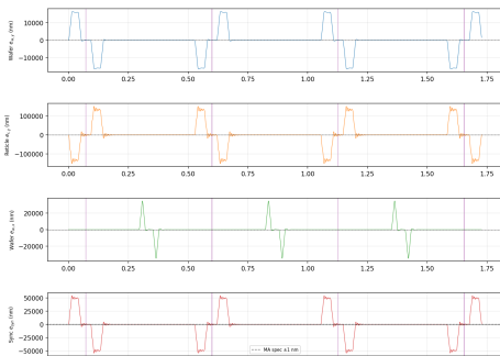
Case 1 — End-Effector Tracking Errors (No Fine Stages) Shaded bands = exposure windows
