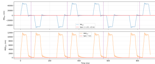
Case 1 — Synchronisation Error Performance Indices (Moving average and MSD over T_{exp} = 1.72 ms window)
