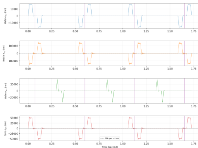
Case 1 — End-Effector Tracking Errors (No Fine Stages) Shaded bands = exposure windows
