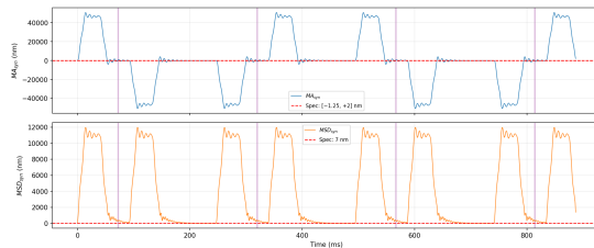
Case 1 — Synchronisation Error Performance Indices (Moving average and MSD over T_{DIO} = 1.72 ms window)
