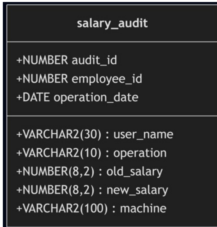
Img 01 - salary_audit TABLE Diagram
