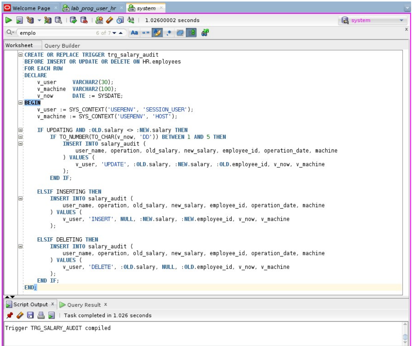
Img 03 - Executes the TRIGGER creation query
