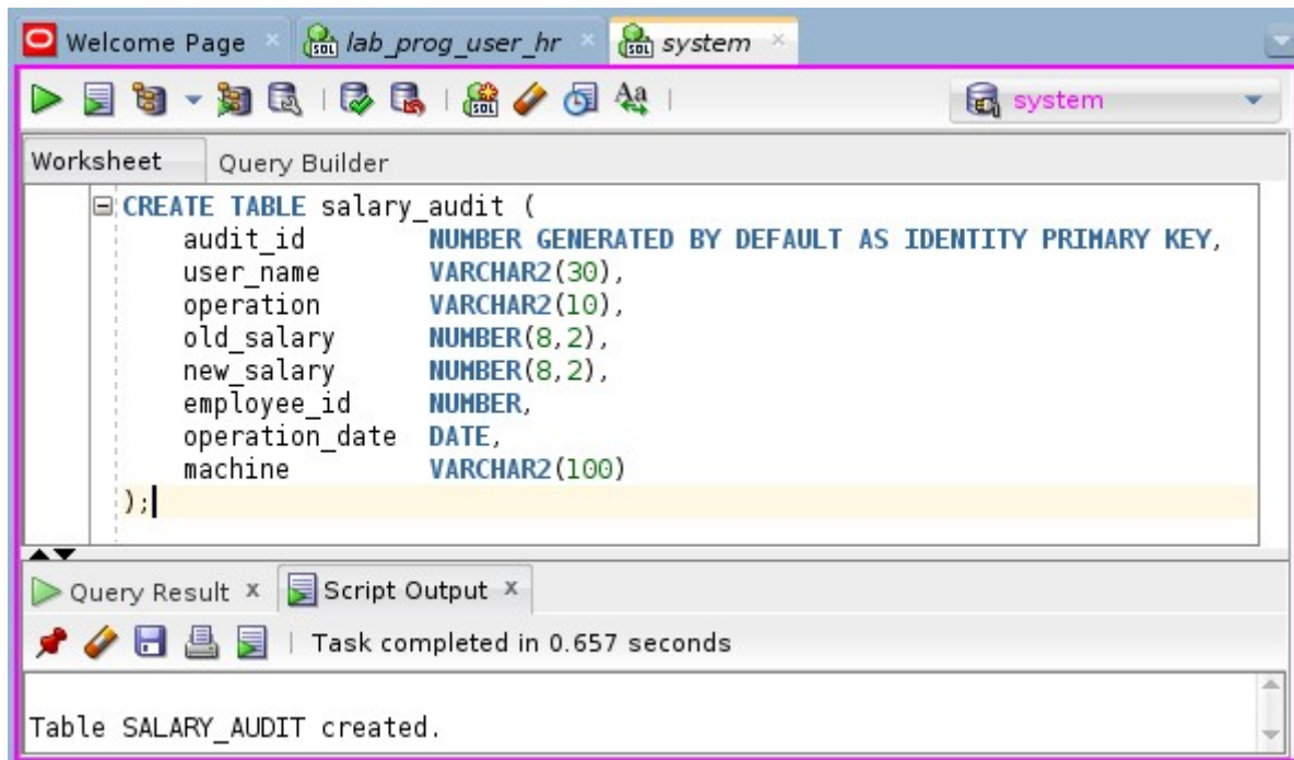
Img 02 - Executes an CREATE TABLE query
